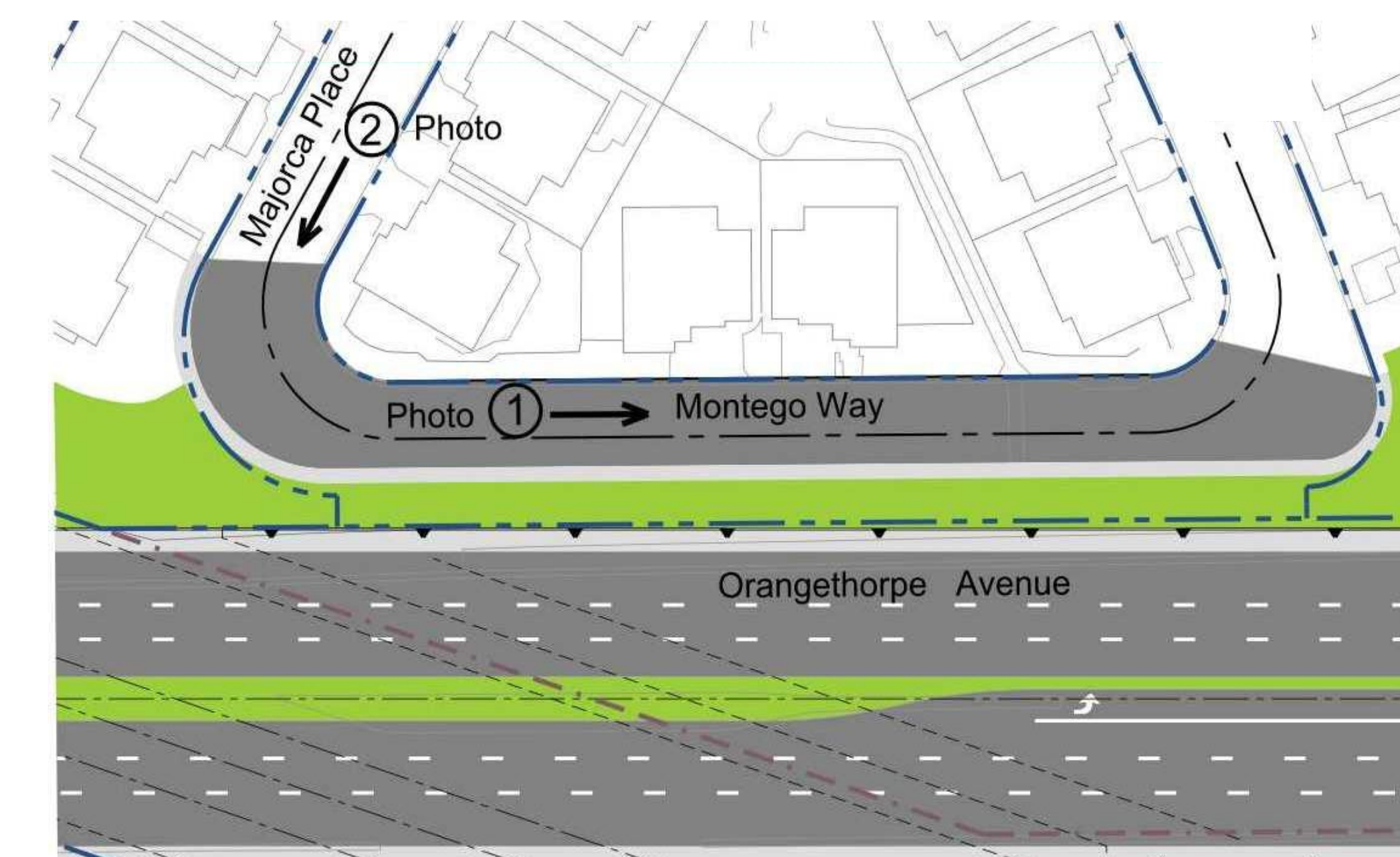
Plan
