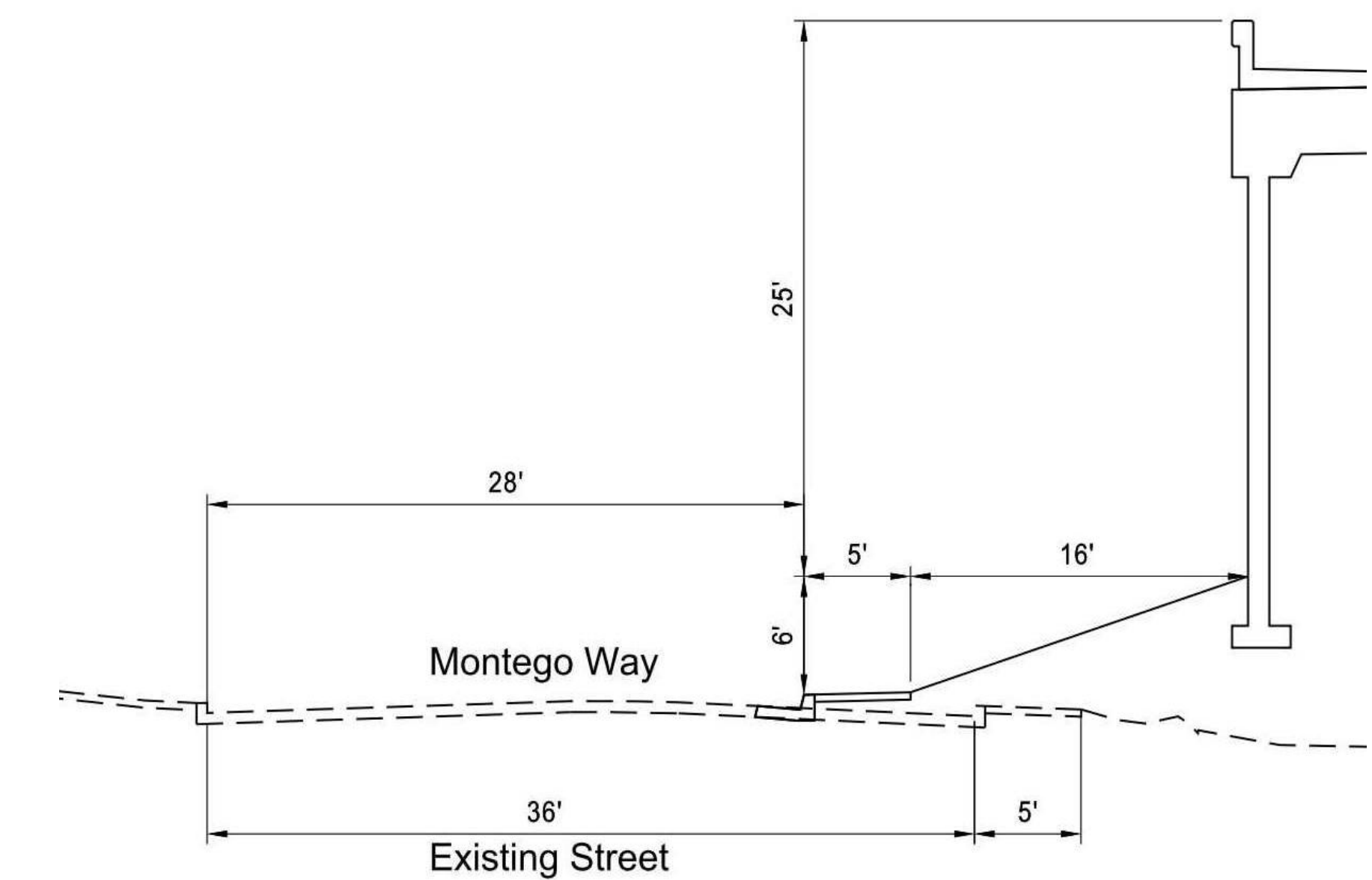
Section
